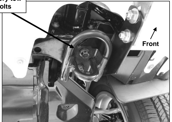
(Fig 4) Driver/left mounting Bracket installation
