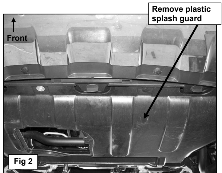
Tow hook mounting location pictured through opening in front bumper cover
