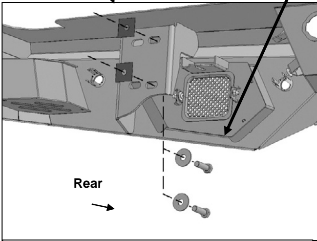
(Fig 17) On 25-3500 models, insert hardware into INNER mounting slots. Thread Plastic Retainers onto Hex Bolts to hold Bolts in place
