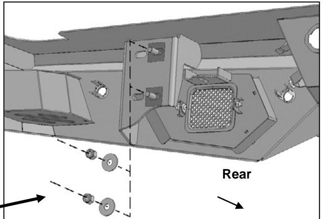
(Fig 18) Attach Bumper to end of frame (passenger/right side of 1500 model illustrated)
